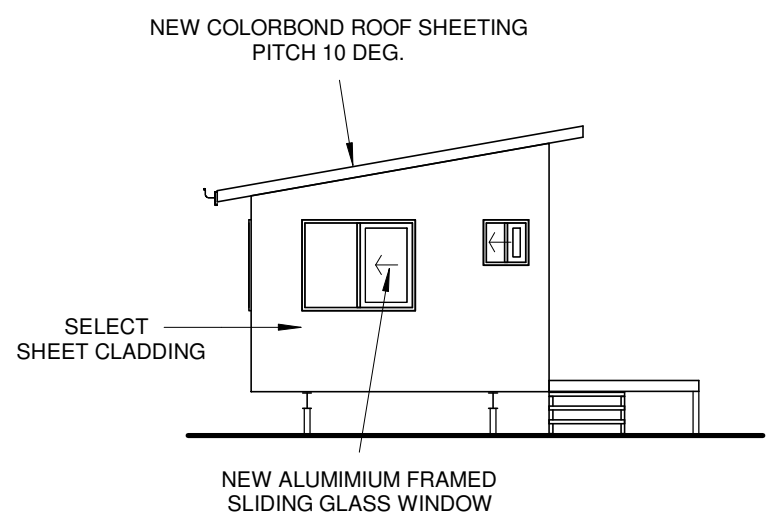
REAR ELEVATION 1:100
