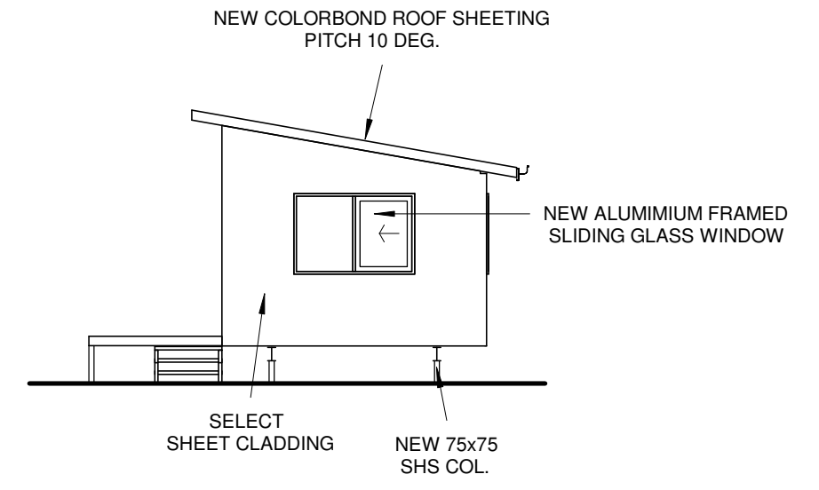
FRONT ELEVATION 1:100
