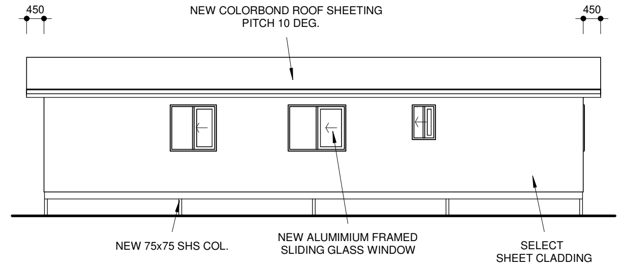
SIDE ELEVATION 1:100
