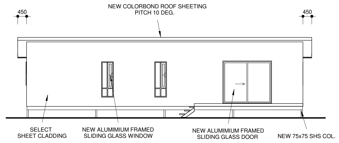
SIDE ELEVATION 1:100
